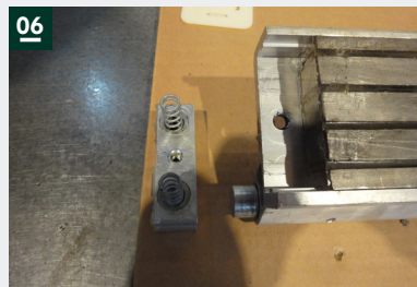
06: Faulty foot block disassembled
