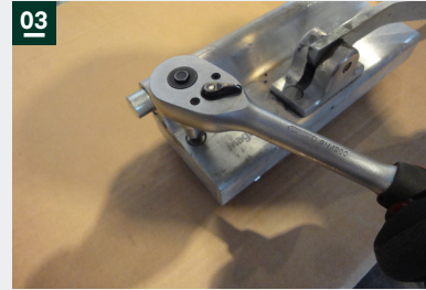
03: Loosen and remove the fixing screw
