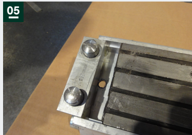
05: Stop at this disassembly point and remove the foot block by hand
