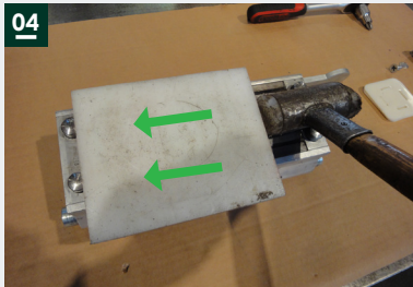
04: Use hammer and tools to loosen the foot block carefully
